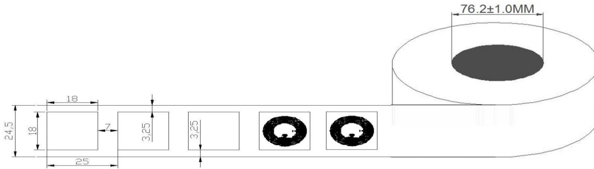
Un-winding Direction/Label Facing Outside 出卷方向图
